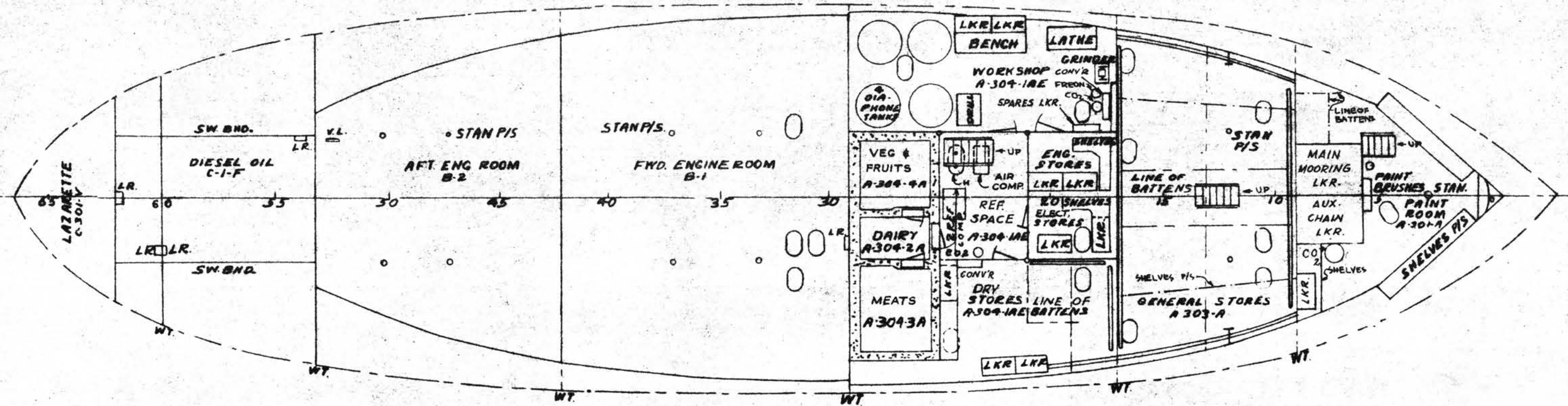
PLATFORM DECK
